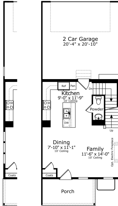
End Unit Main Level
