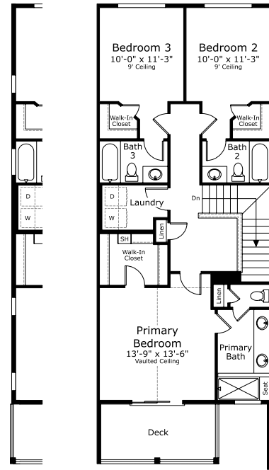
End Unit Upper Level
